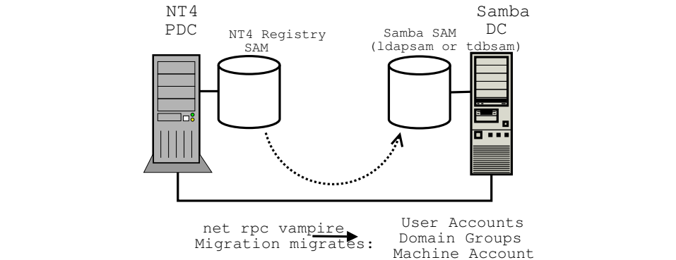
Figure 9.1 Schematic Explaining the net rpc vampire Process
