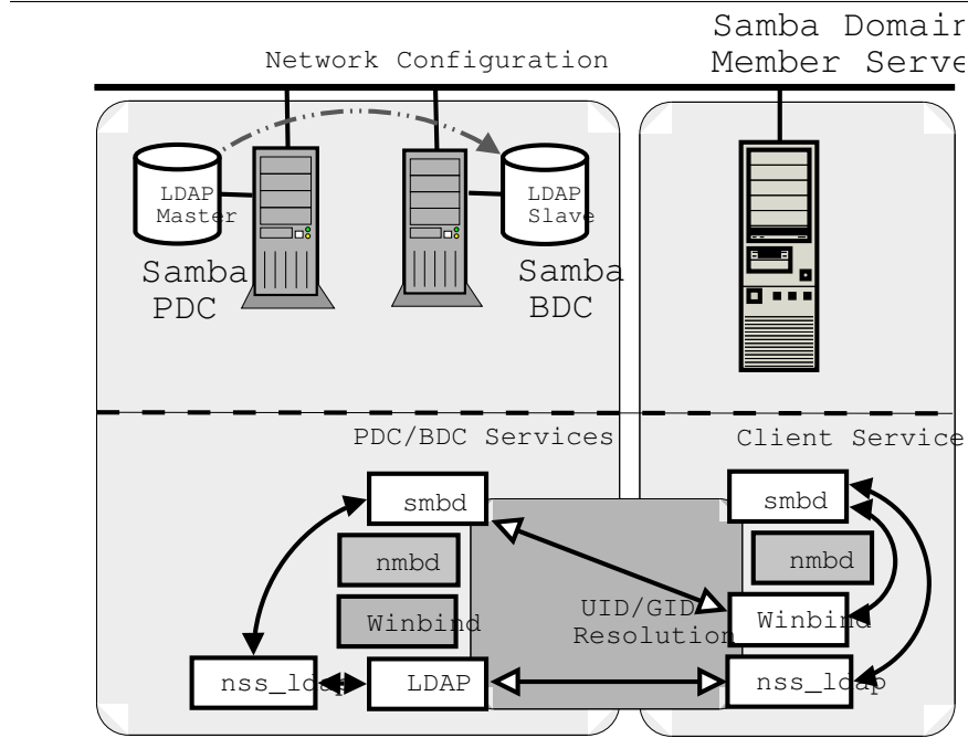
Figure 7.2 Samba Domain: Samba Member Server
