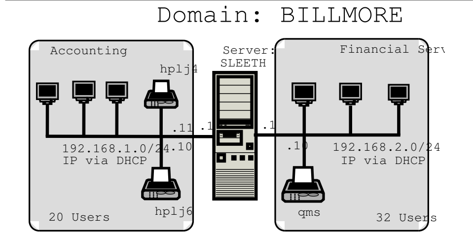
Figure 2.1 Abmas Accounting — 52-User Network Topology
