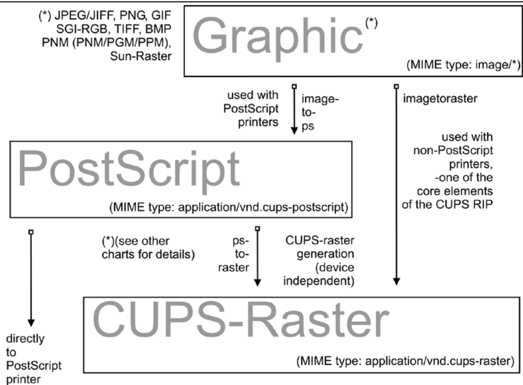
Figure 19.8: Image format to CUPS-raster format conversion.
