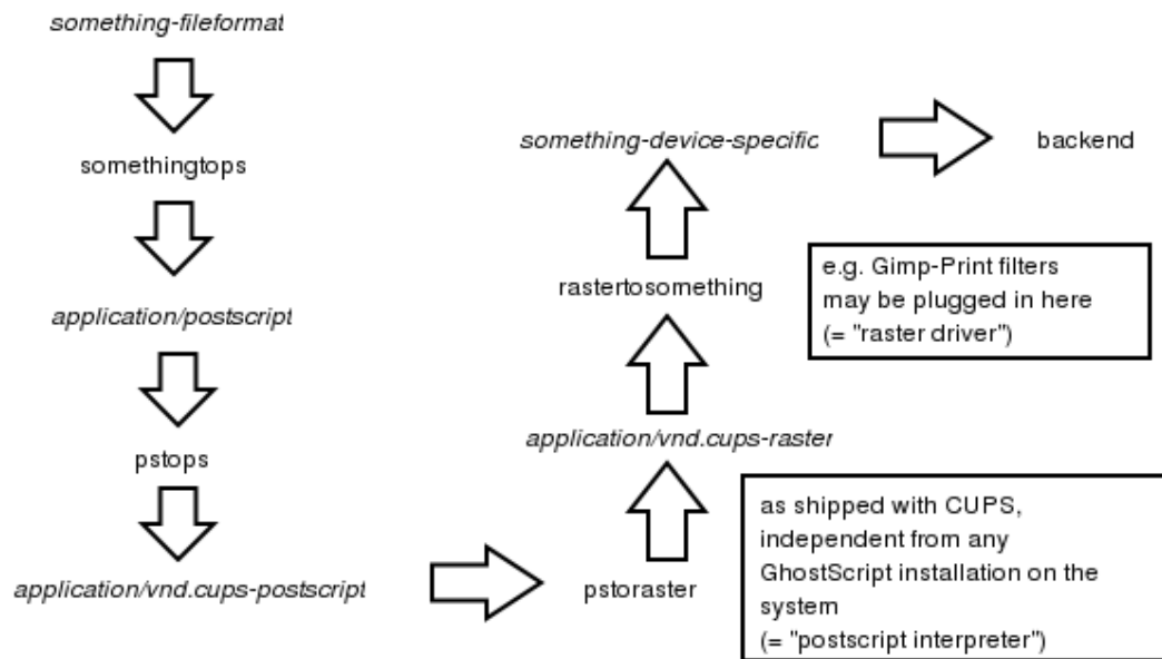
Figure 19.17: Filtering chain 1.
